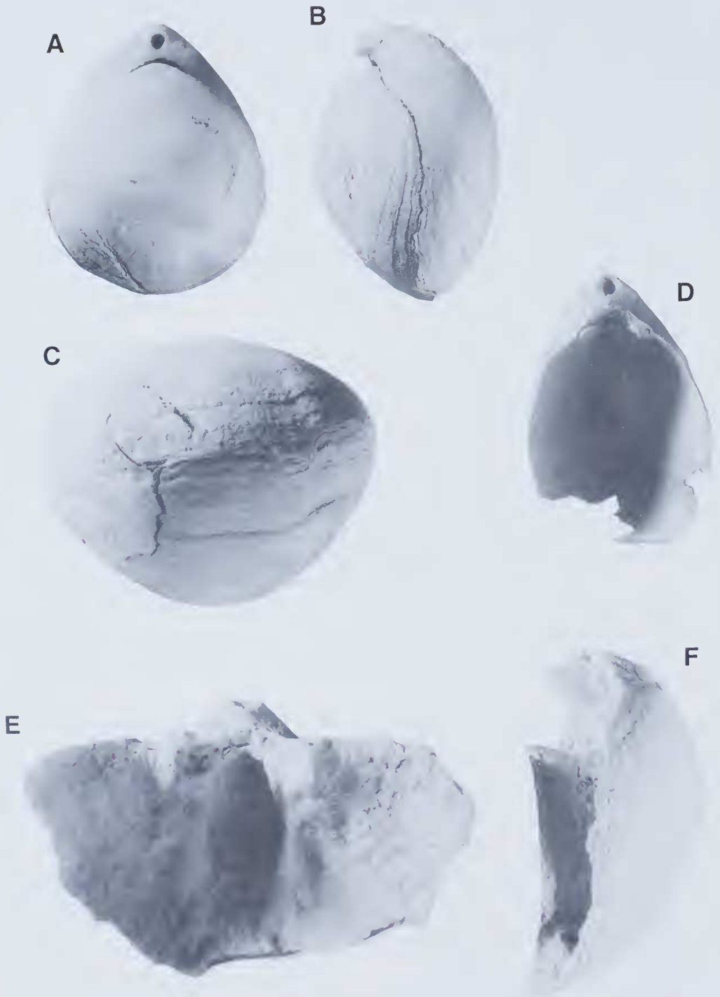
Figure 3 Neothyris rylandae A, WAM 82.2368, Holotype, dorsal valve exterior \times 1 ; B, WAM 82.2368, Holotype, lateral margin \times 1 ; C, WAM 82.2368, Holotype, anterior commissure \times 1.5 ; D, WAM 82.2378a, Paratype, ventral valve interior \times 1 ; E, WAM 82.2367b, Paratype, ventral valve interior \times 2.5 ; F, WAM 82.2367a, lateral view of the brachial valve \times 1.5 .
